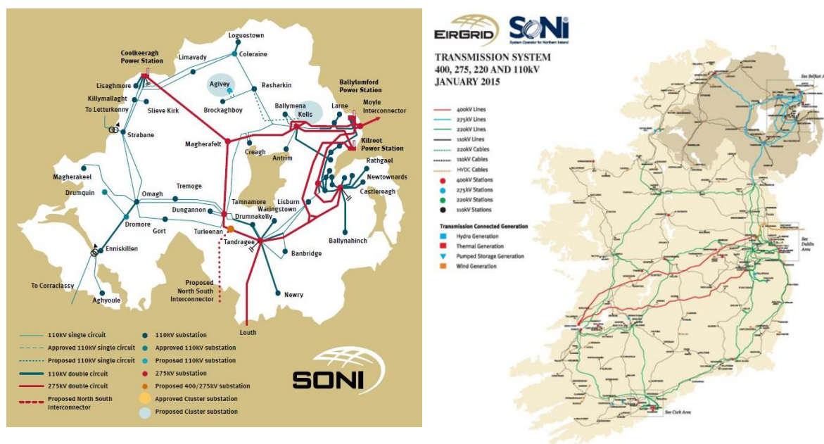
Figure 8: Northern Ireland & Ireland Electricity Transmission System
