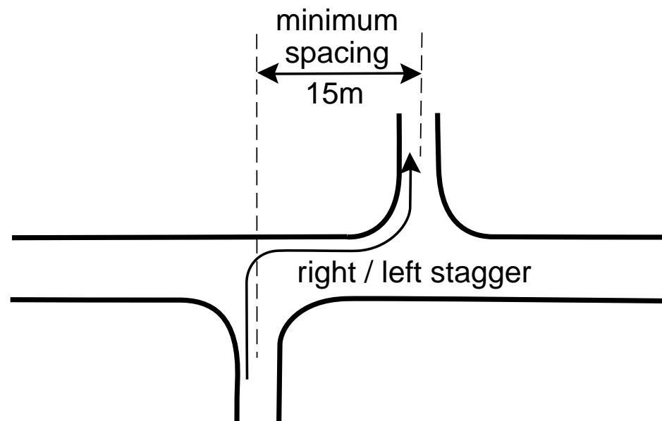
Fig 5: Right / left junction stagger
