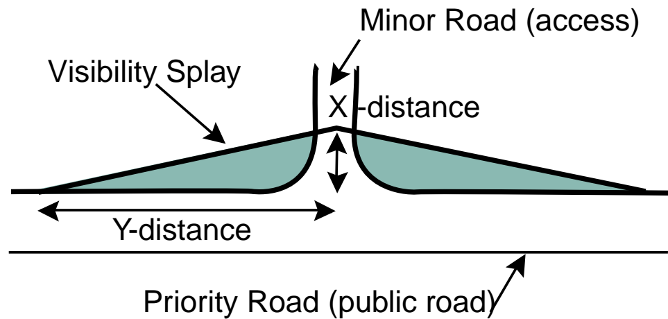
Fig 1: Visibility Splays
