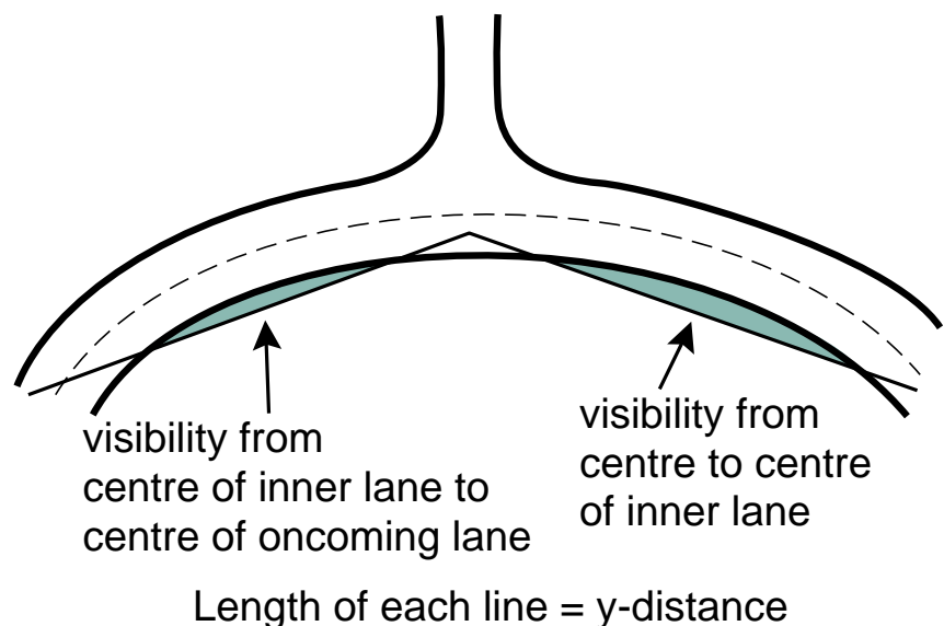
Fig 3: Forward Visibility Requirements
