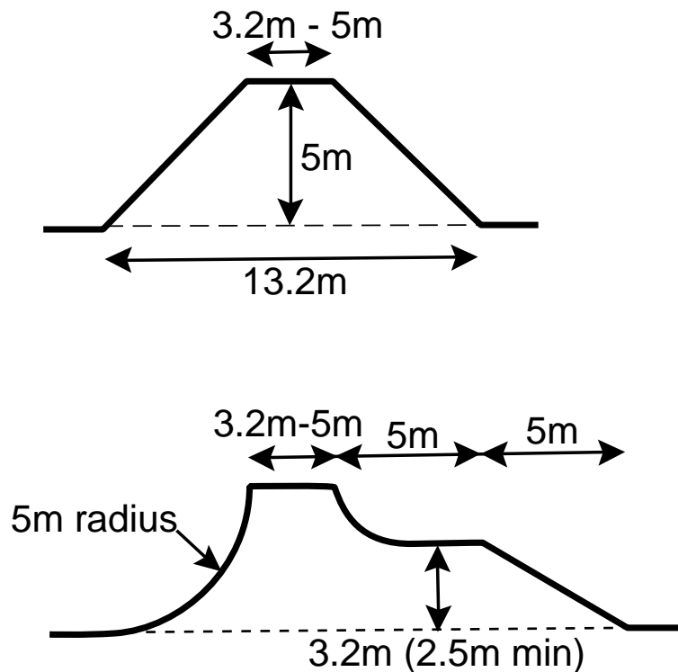
Fig 6: Alternative Layouts for Rural Accesses
